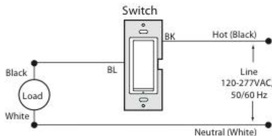
MWSS10-G (No Neutral)
