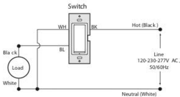
MWSS10 (With Neutral) Mx-ILS2 (With Neutral)
